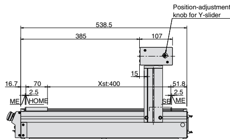
Position-adjustment knob
