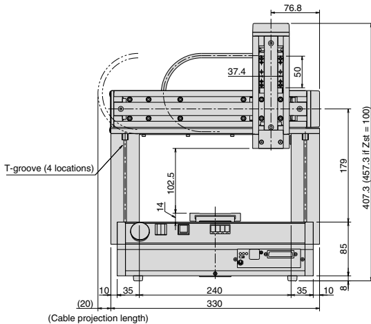
Z-axis slider installation hole
