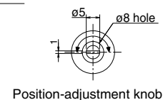
Position-adjustment knob
