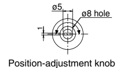
Position-adjustment knob
