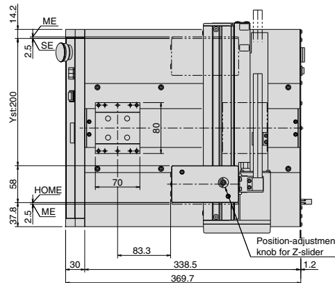
Z-axis slider installation hole
