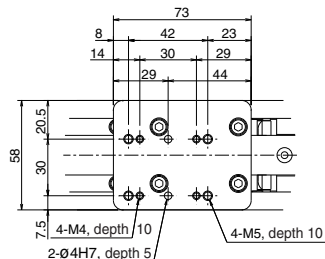
Y-axis slider installation hole
