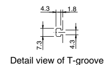
Detail view of T-groove
